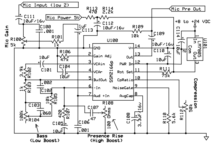
100 - Microphone Preamp / Compressor (Preamp Board)
